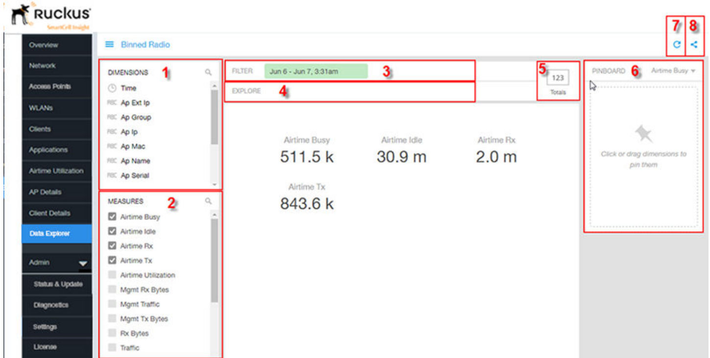
FIGURE 116 Data Cube Filters
