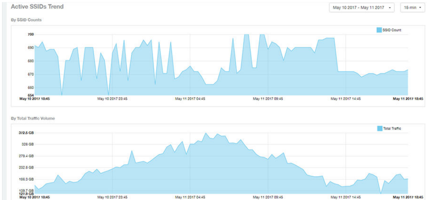
FIGURE 61 WLANs - Active SSIDs Trend Graphs
