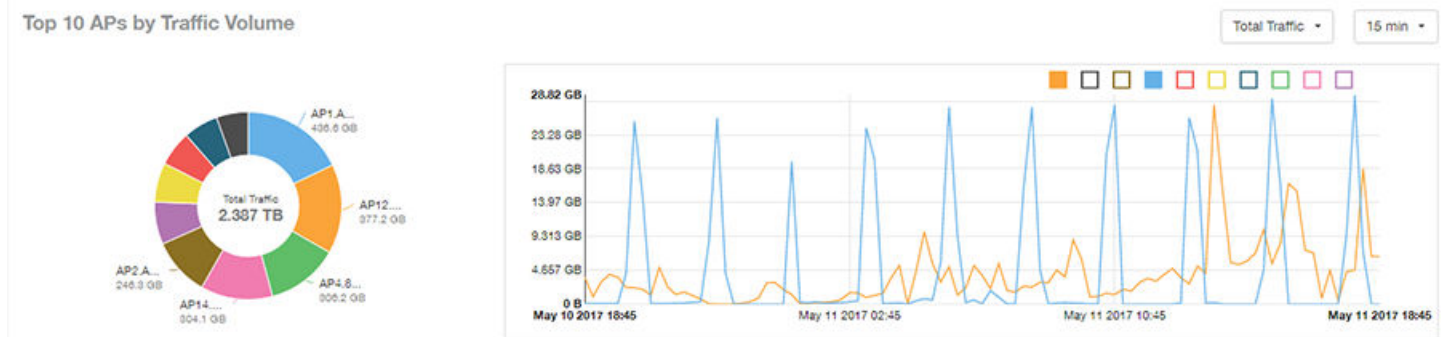
FIGURE 35 Network - Top 10 APs by Traffic Volume
