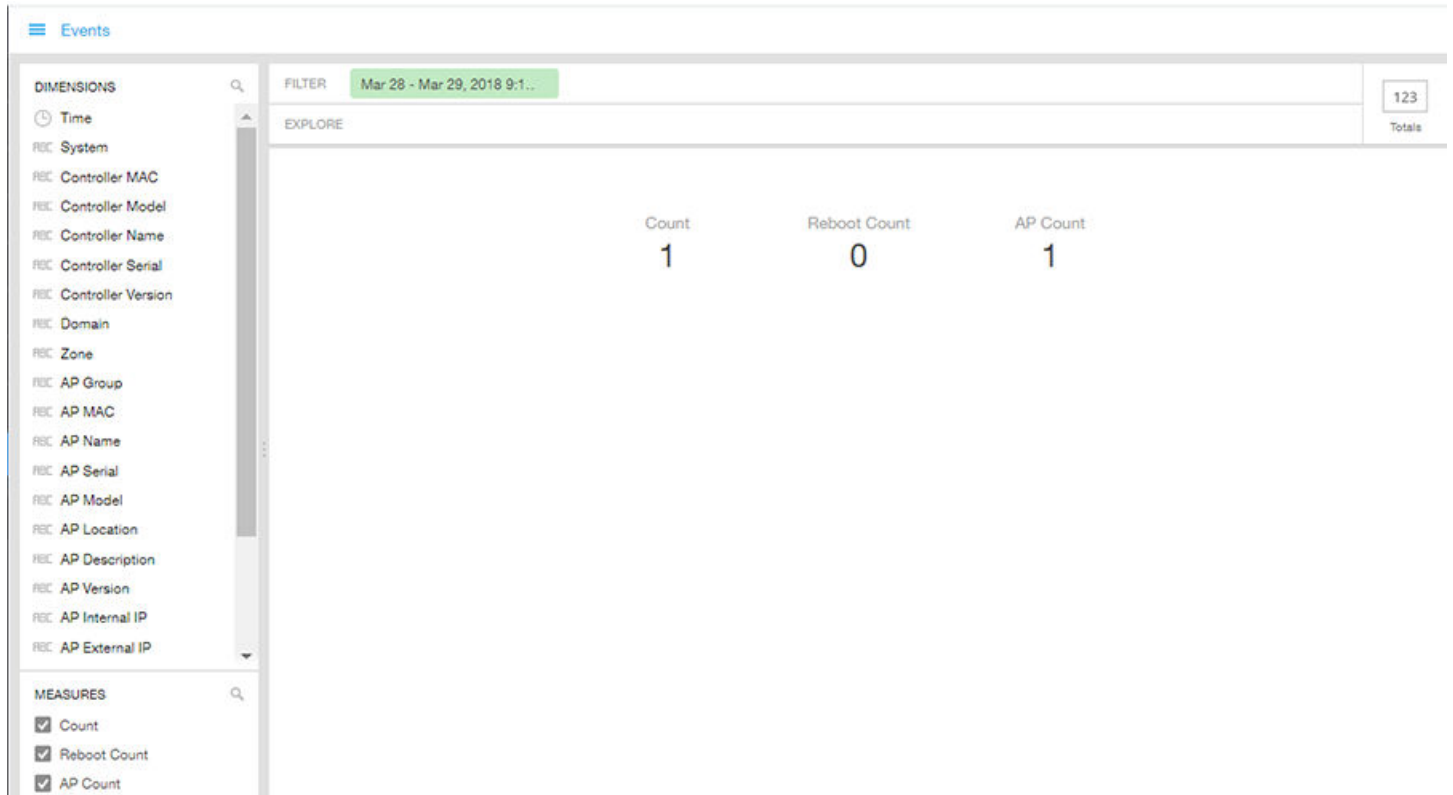
FIGURE 112 Data Explorer - Events
